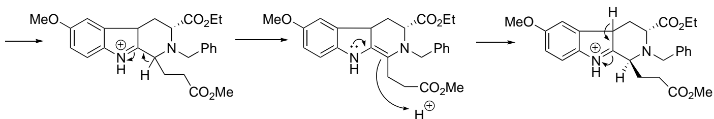
Pictet-Spengler Synthesis
