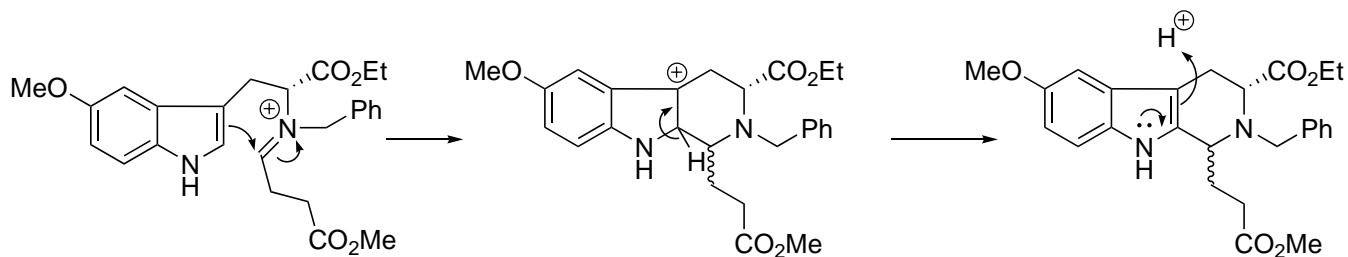
Pictet-Spengler Synthesis
