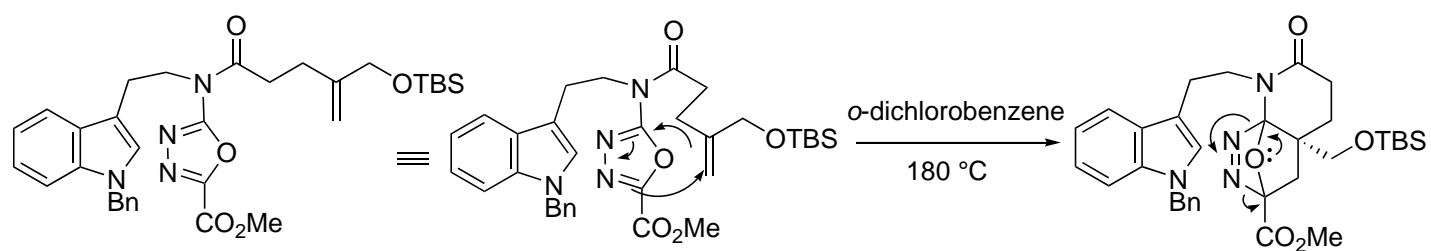
Hetero Diels-Alder reaction
