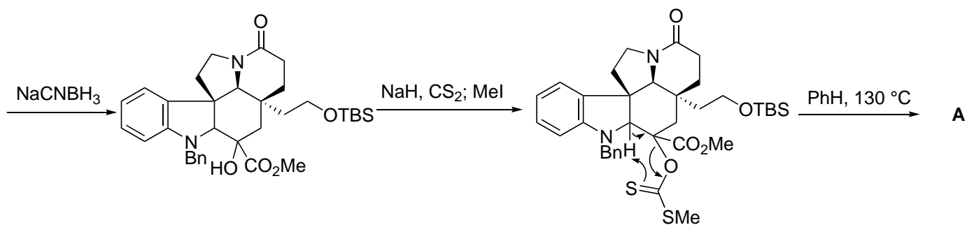
Chugaev Elimination reaction
