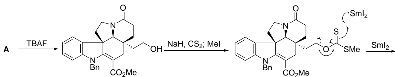
Chugaev Elimination reaction
