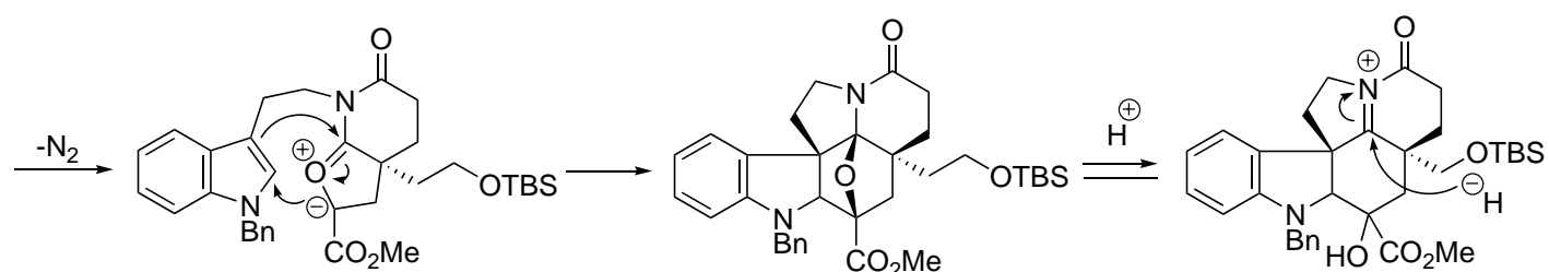
1,3-Dipolar Cycloaddition
