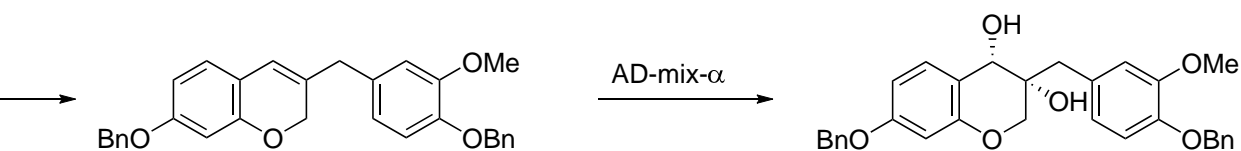
Sharpless asymmetric dihydroxylation
