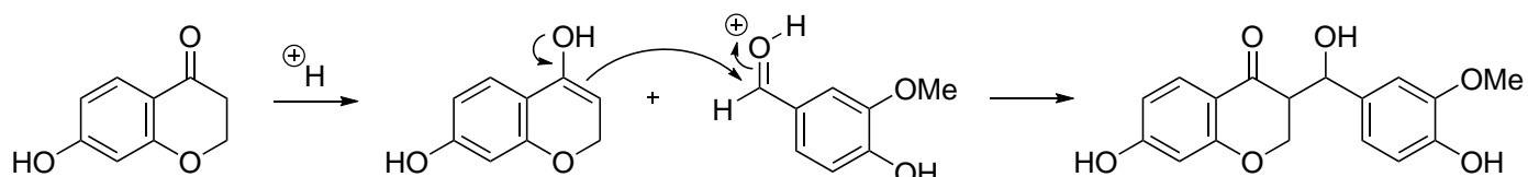
Claisen-Schmidt reaction
