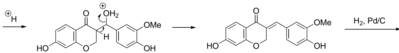
Claisen-Schmidt reaction
