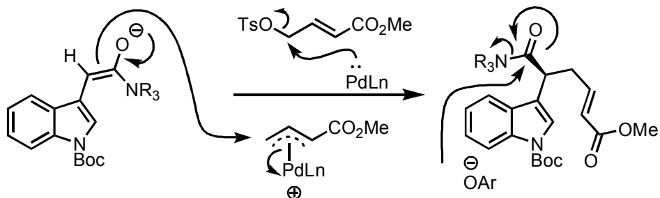
Tsuji-Trost reaction
