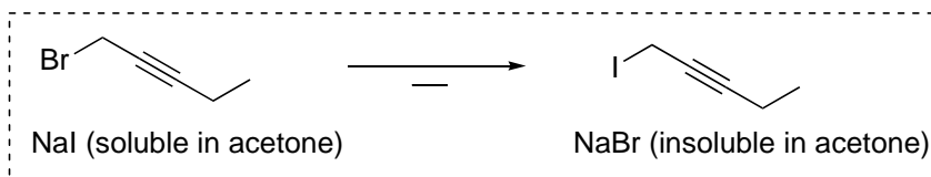
Finkelstein Reaction
