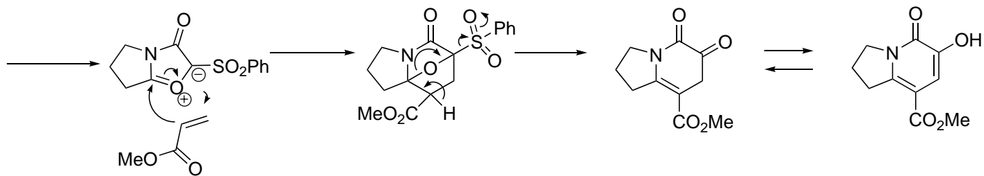
1,3-Dipolar Cycloaddition
