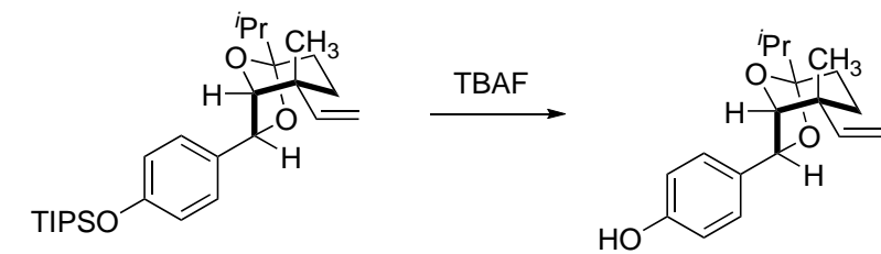
Barton Radical Decarboxylation Reaction
