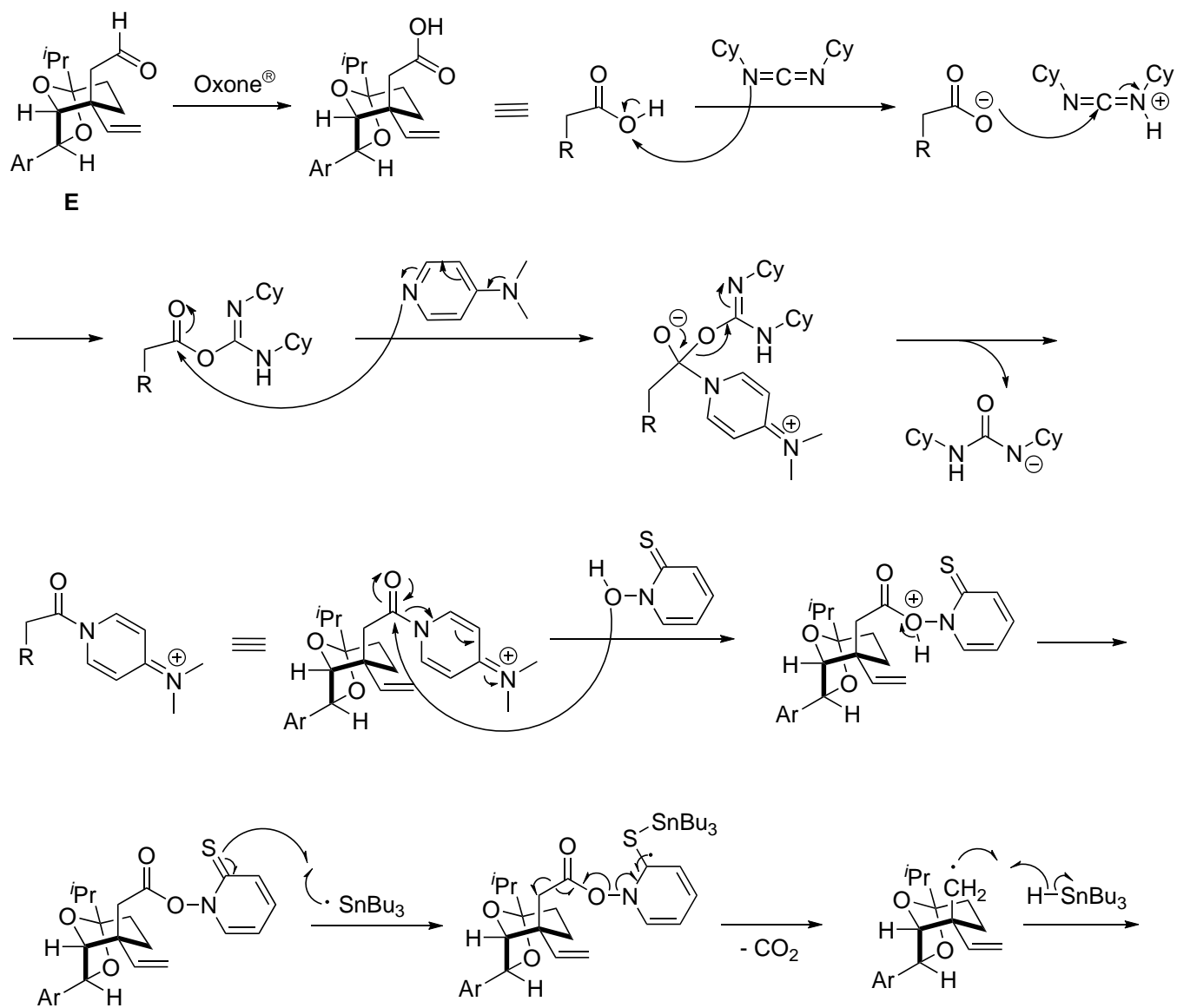
Barton Radical Decarboxylation Reaction
