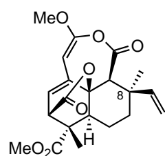
basiliolide B (5%)
