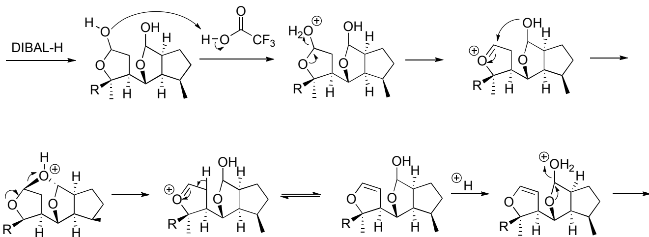
Retro-Claisen condensation
