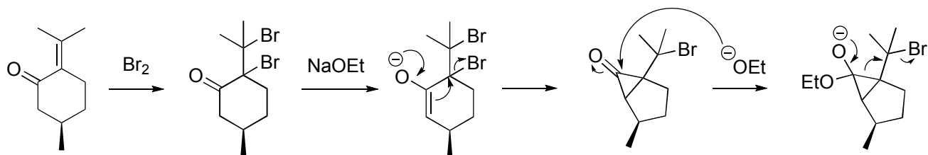
Favorskii Rearrangement
