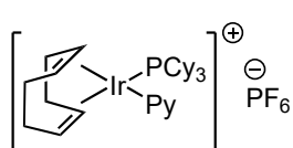
Crabtree's catalyst
